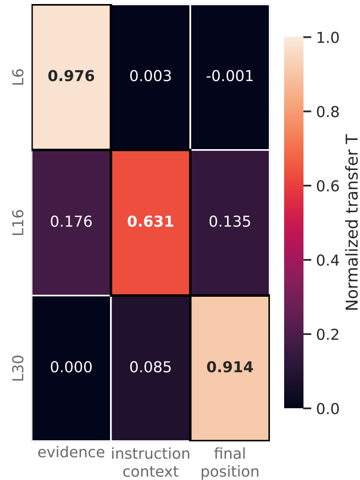
(b) Held-out confirmation (frozen 3\u00d773)
