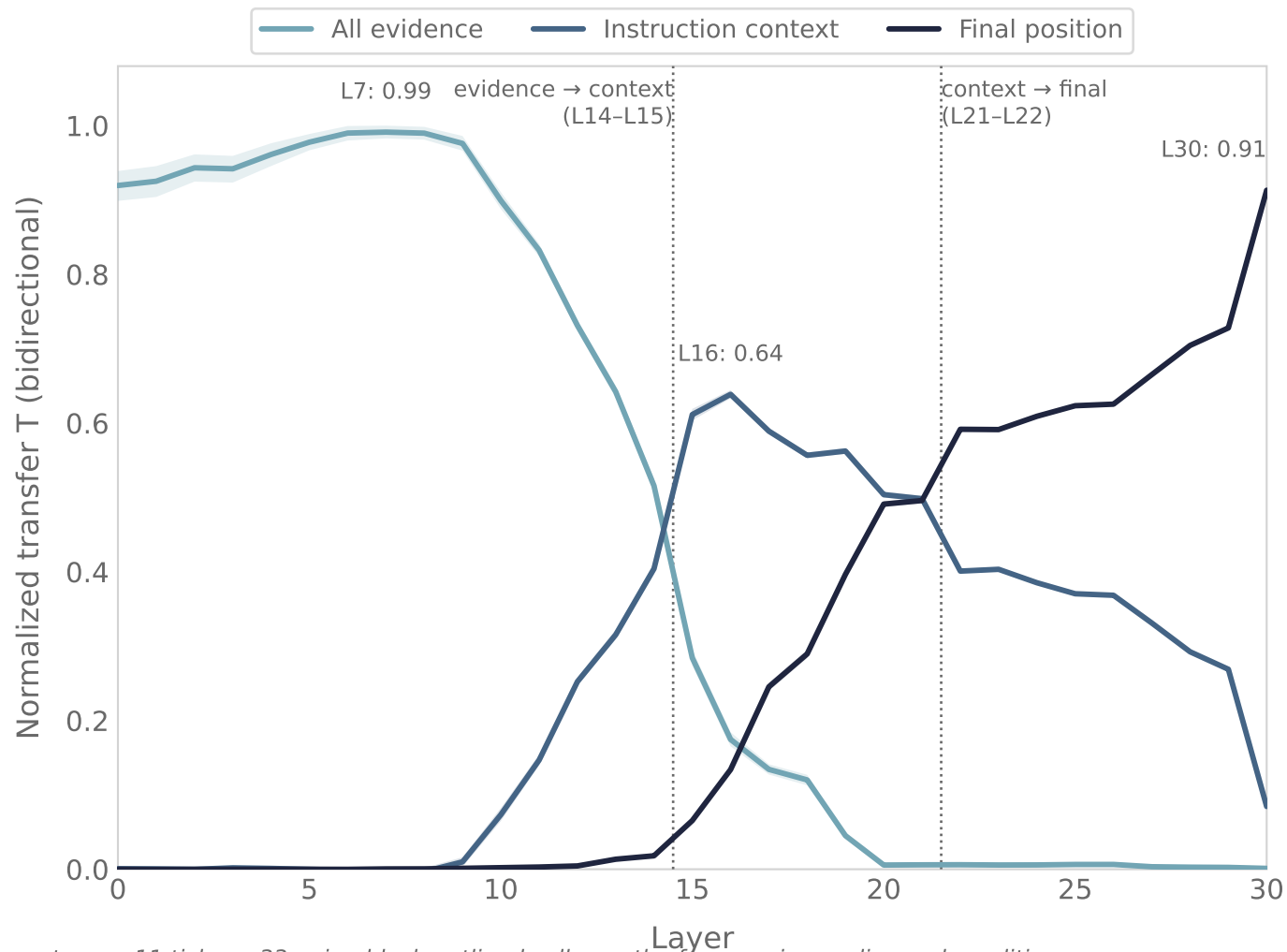
(a) Discovery: source-outcome sufficiency by span and layer
