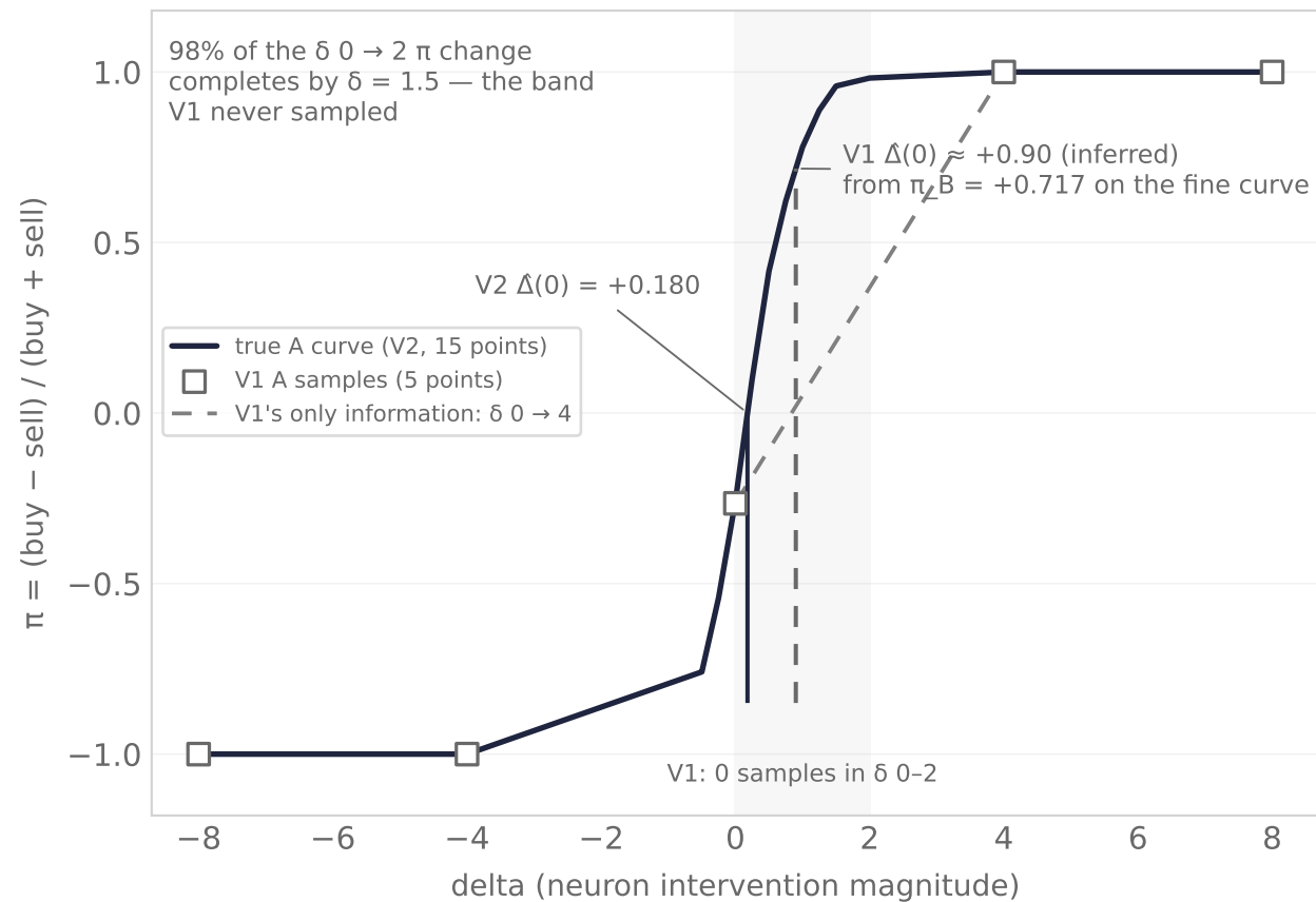
(a) V1's five A samples vs the true curve
