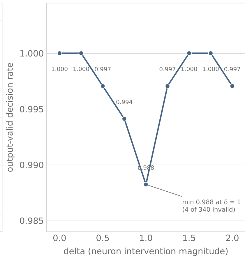
(b) validity across the fine grid
