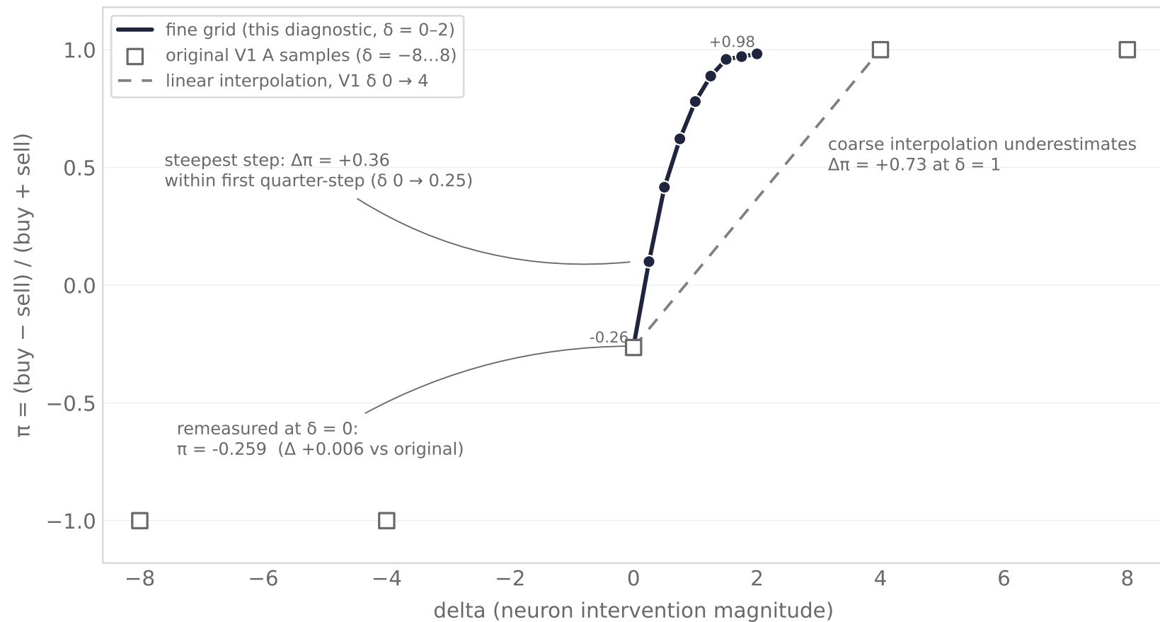
(a) \pi response across the delta grid
