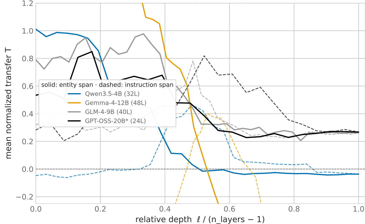
Cross-model Phase 2B — entity-state layer sweep by relative depth (frozen shared-evidence template, 16 companies, 8 transfer directions; *GPT-OSS-20B is MoE, shown as requested exception)
