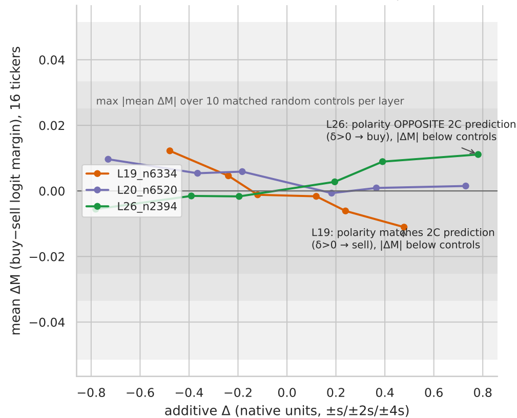
(a) Candidate coordinates — \Delta M vs \Delta (all positions)
