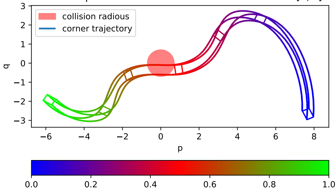
Obstacle position in the Frenet frame w.r.t time t \in [0; 1]
