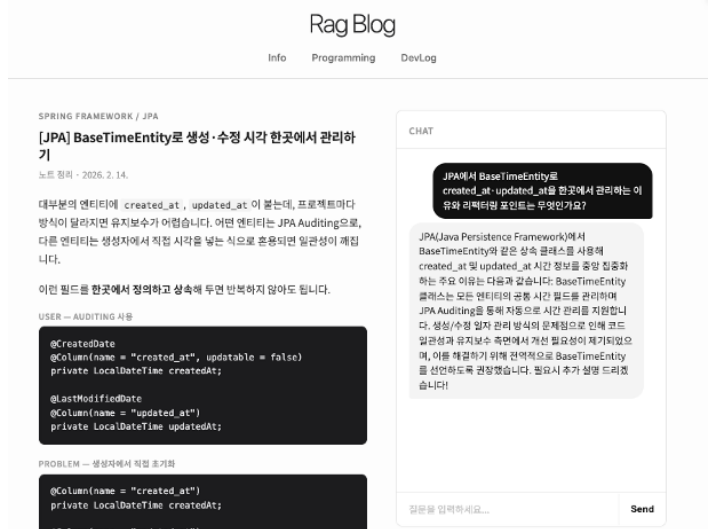
Fig1. Implementation of RAG Chatbot for Tech Blog
