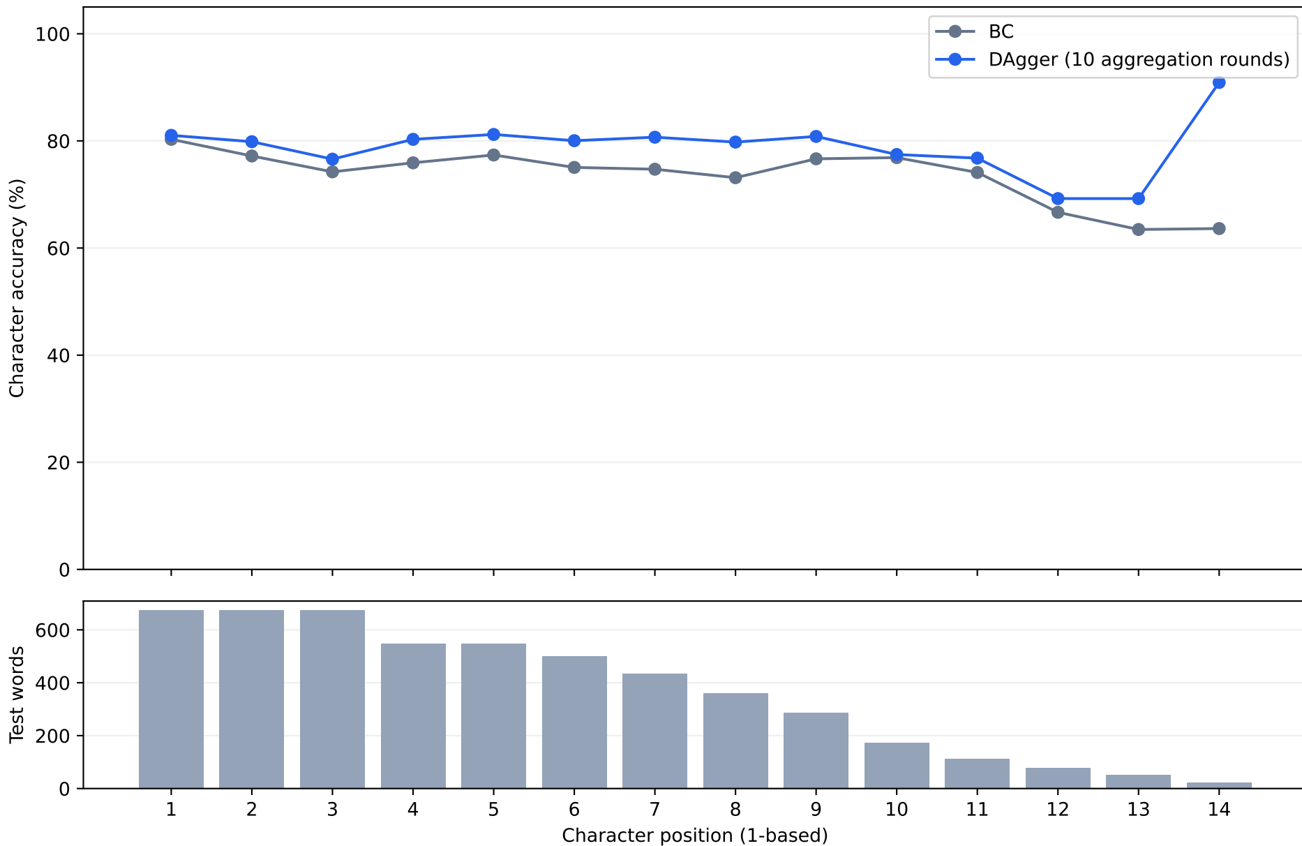
Ablation D: free-running accuracy by position Test fold 9, seed 0
