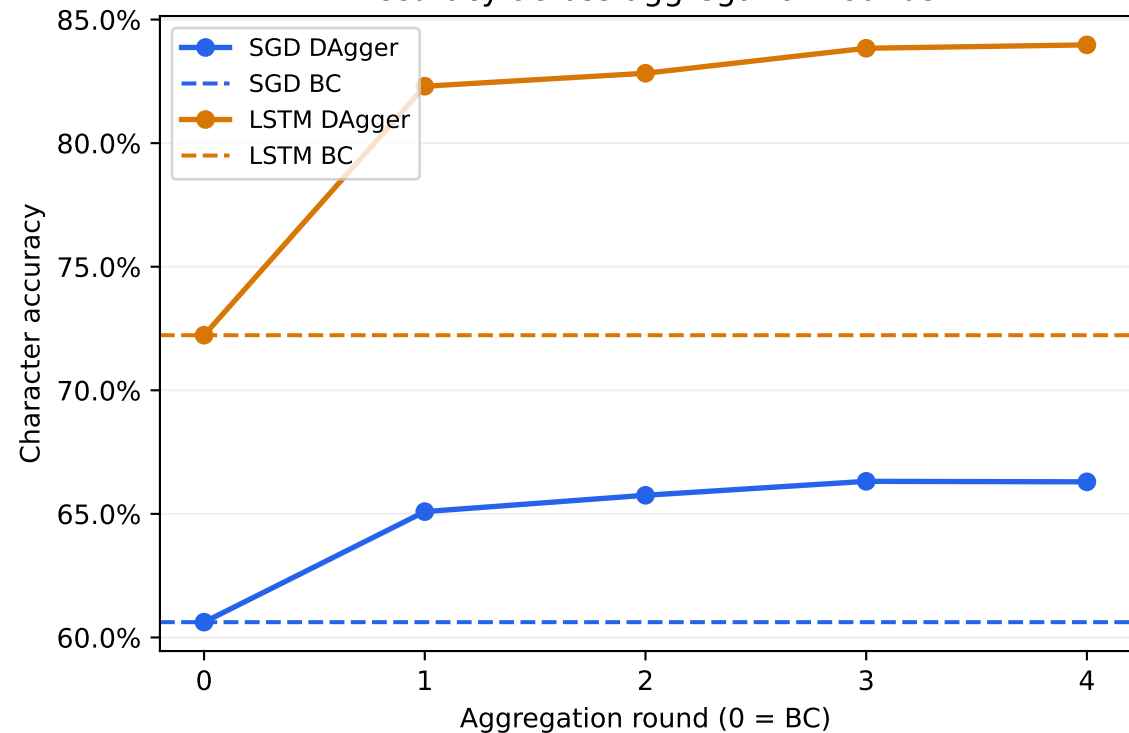
Accuracy across aggregation rounds
