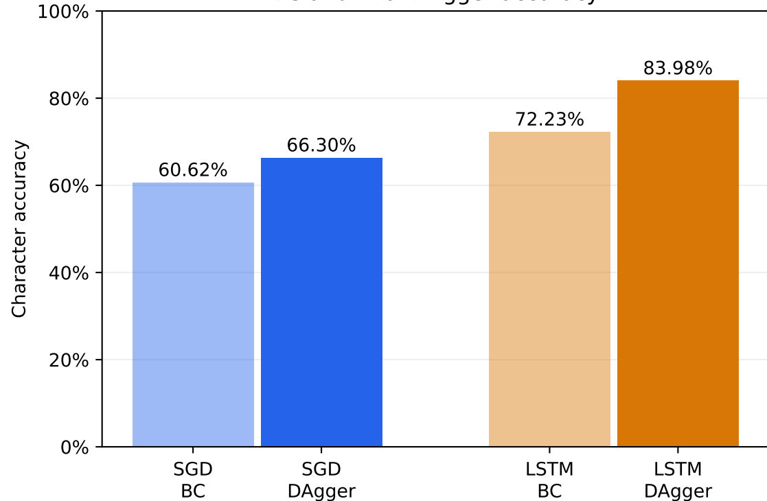
BC and final DAgger accuracy
