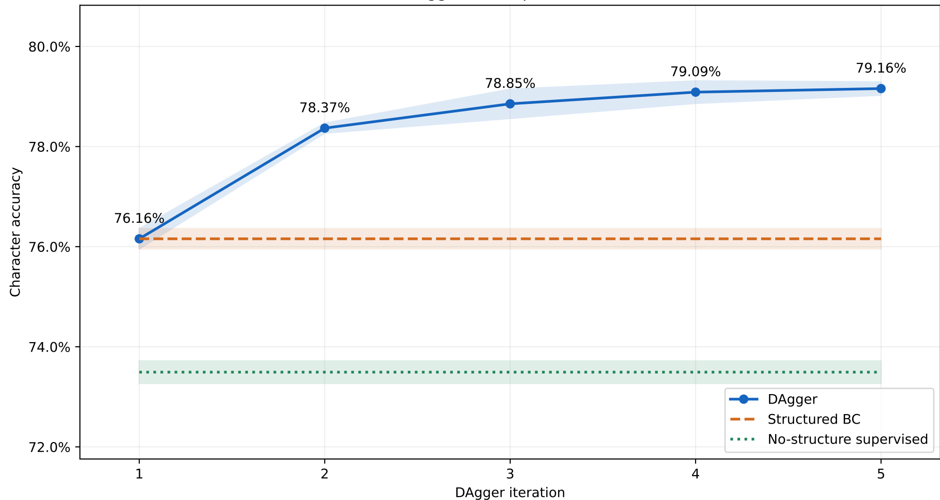
Stanford OCR: DAgger and supervised baselines (fold 9)
