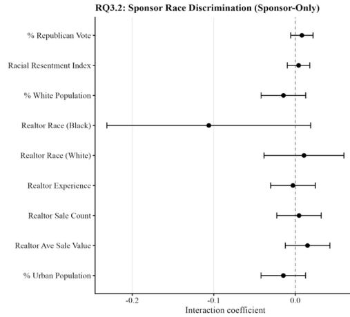
Figure S58: Pre-registered Heterogeneity: RQ3.2
