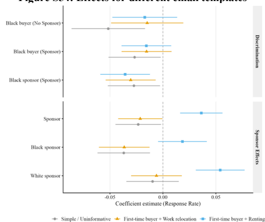
Figure S54: Effects for different email templates
