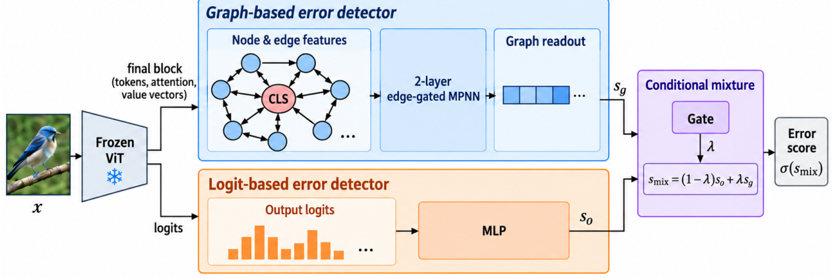
Figure 1: Overview of Polygraph. A frozen ViT supplies a final-block token graph and output logits. A two-layer edge-gated MPNN and an output MLP produce error scores s_g and s_o , combined by a conditional mixture gate.
