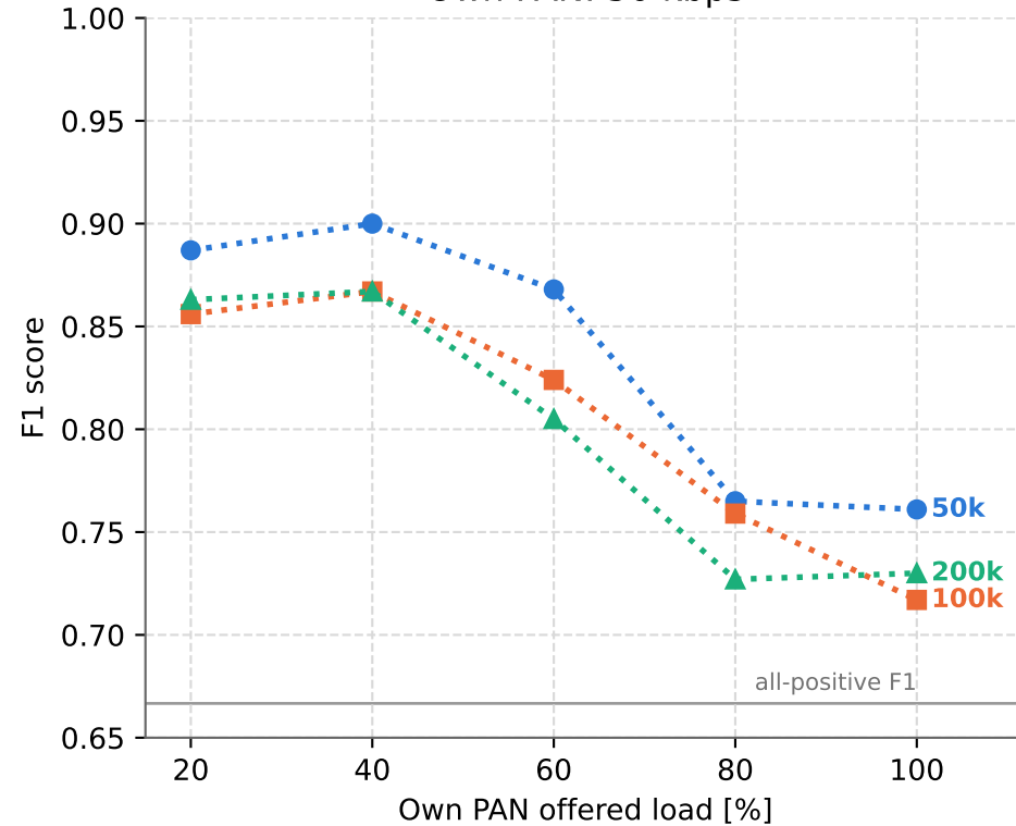
Own PAN: 50 kbps
