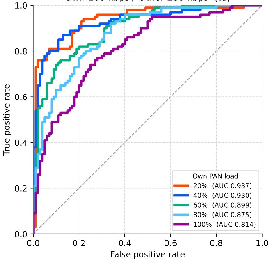
Own 100 kbps / Other 200 kbps (td)
