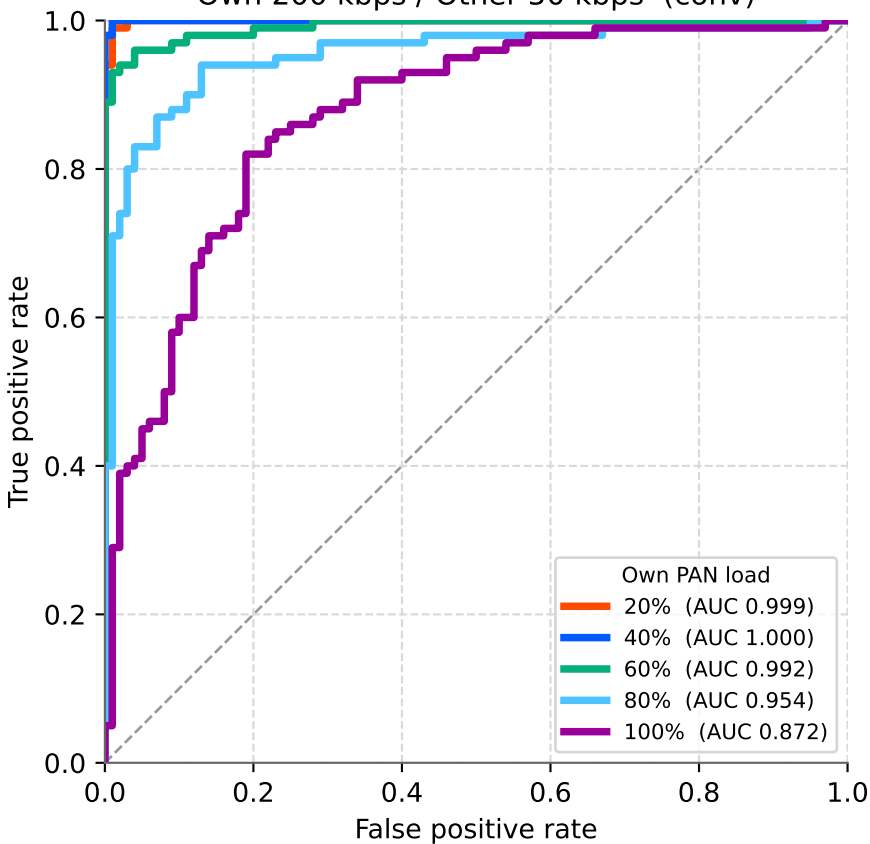
Own 200 kbps / Other 50 kbps (conv)
