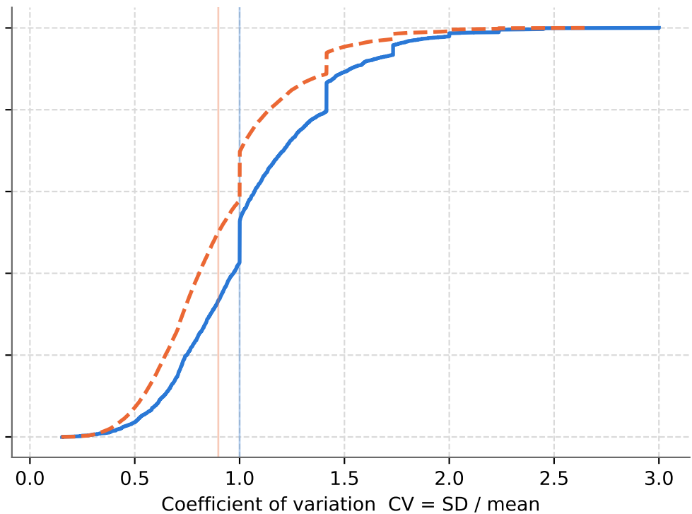
Downlink (DL)
