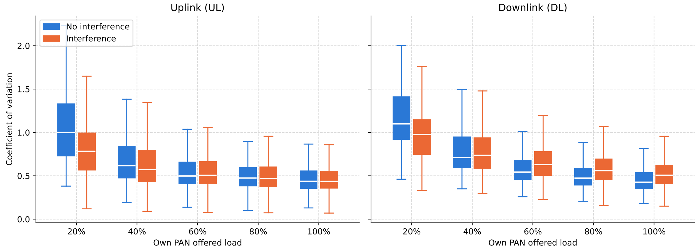
CV by own PAN offered load (whiskers = 1.5 IQR, outliers hidden)
