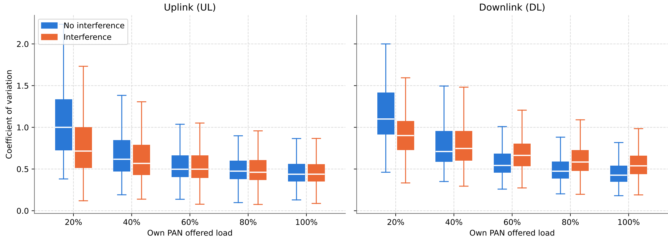
CV by own PAN offered load (other PAN load = 100%) whiskers = 1.5 IQR, outliers hidden
