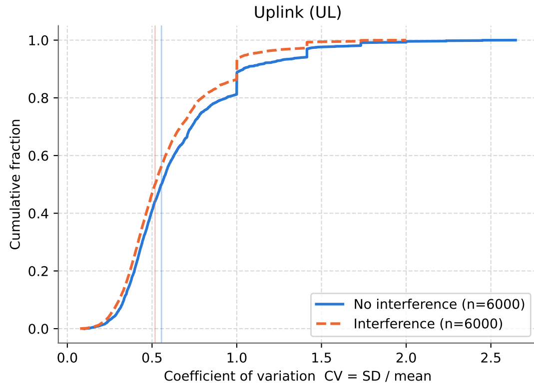
ECDF of CV of PER (aggregate=max, other PAN load = 100%) vertical line = median
