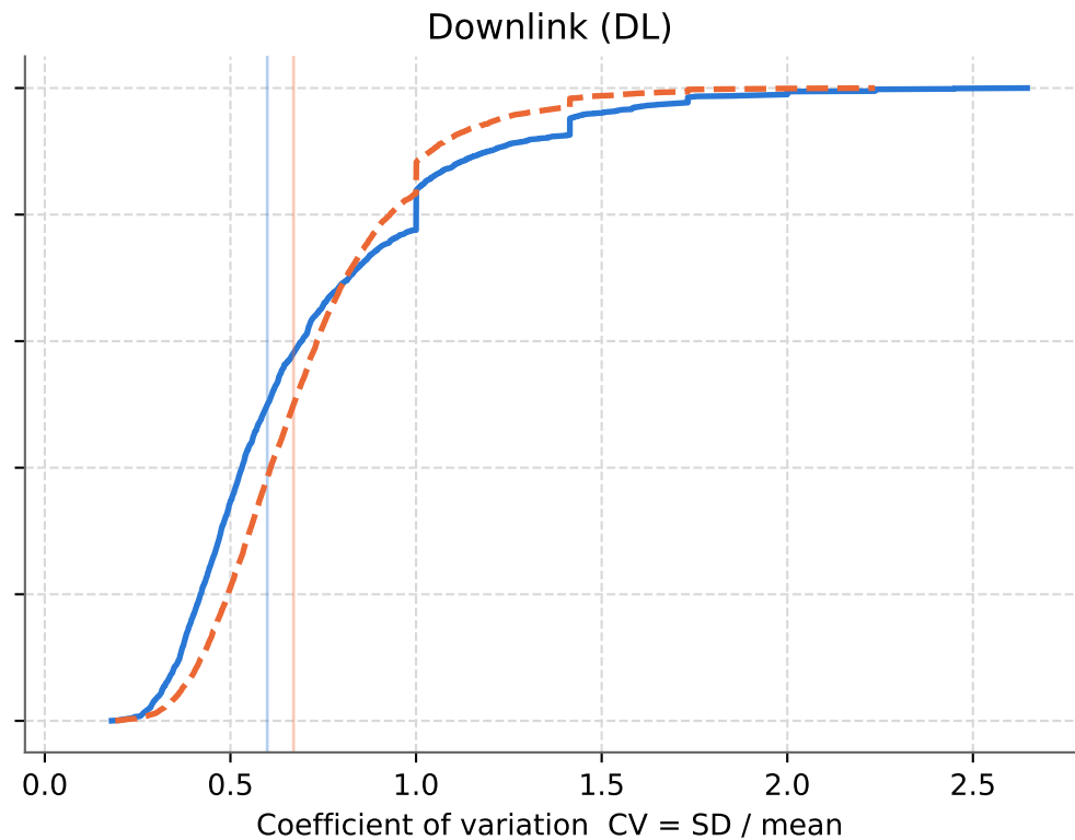
ECDF of CV of PER (aggregate=max, other PAN load = 100%) vertical line = median
