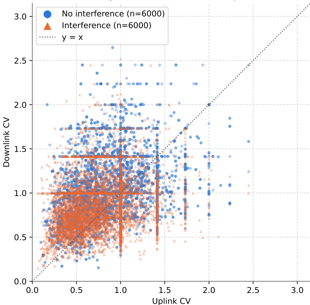
Uplink vs downlink CV (other PAN load = 100%) (above y=x : downlink is more dispersed)
