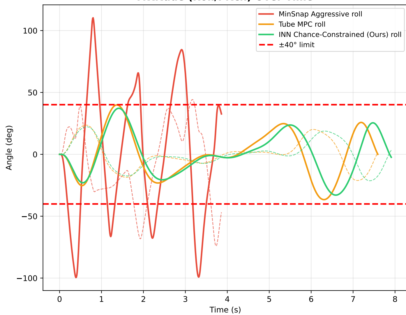
Attitude (Roll/Pitch) Over Time
