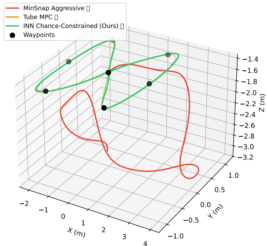
3D Trajectory Comparison (figure8)
