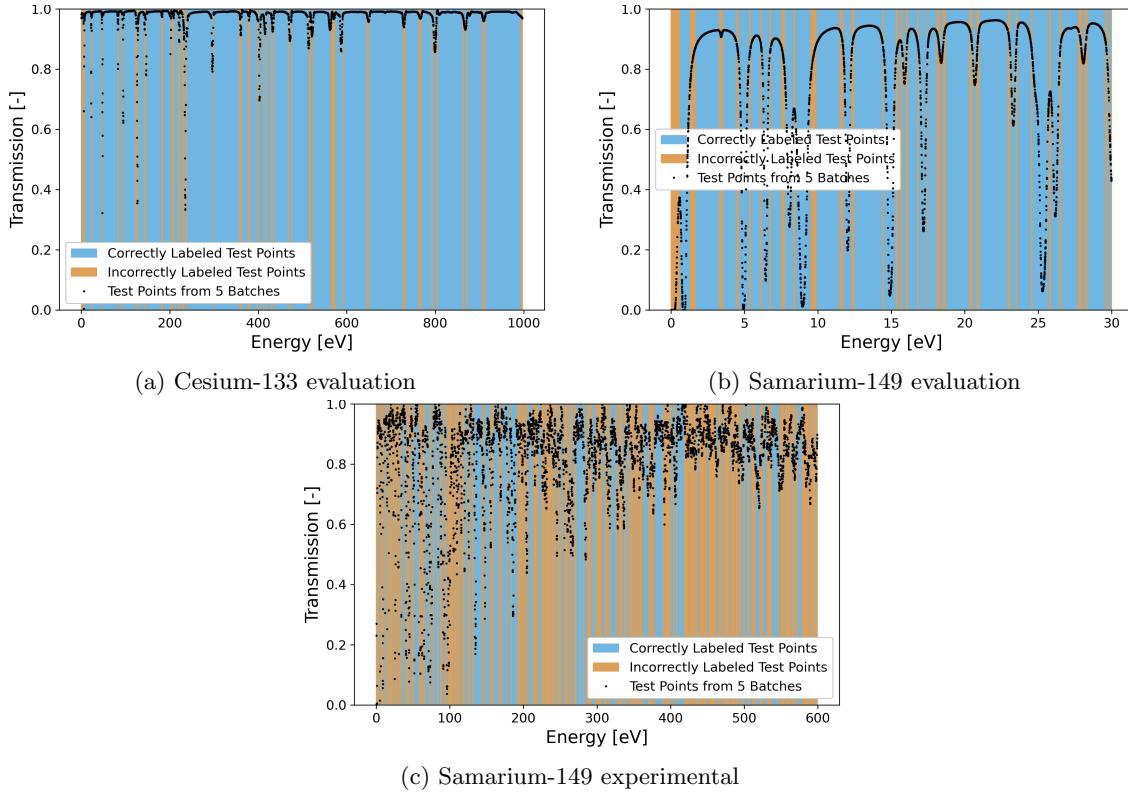
Fig. 5. Model predictions from the first k-fold model on five batches of unseen test data.
