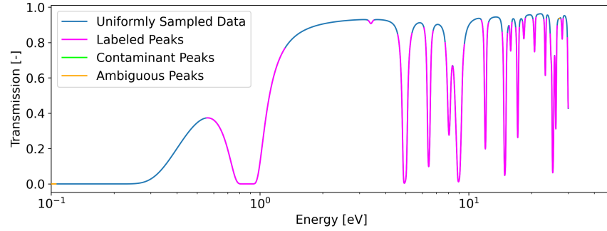
Fig. 3. Samarium-149 evaluation labeled transmission spectrum.
