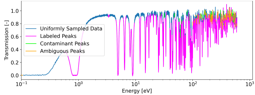
Fig. 4. Experimental Samarium-149 labeled transmission spectrum.
