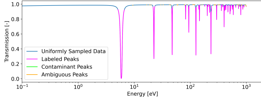
Fig. 2. Cesium-133 labeled transmission spectrum.
