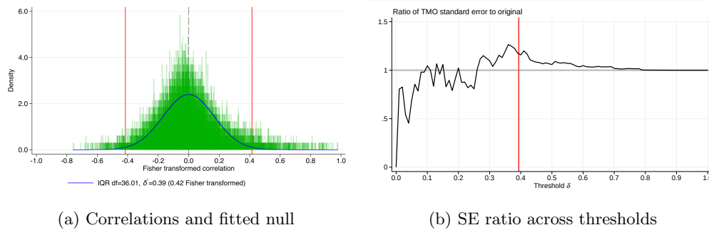
Figure 5: Diagnostics for the application to Acemoglu et al. (2019)
