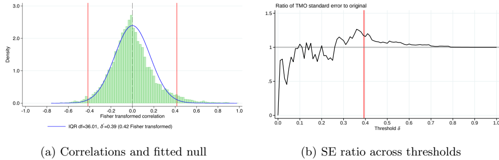
Figure 6: Diagnostics for the application to Acemoglu et al. (2019)
