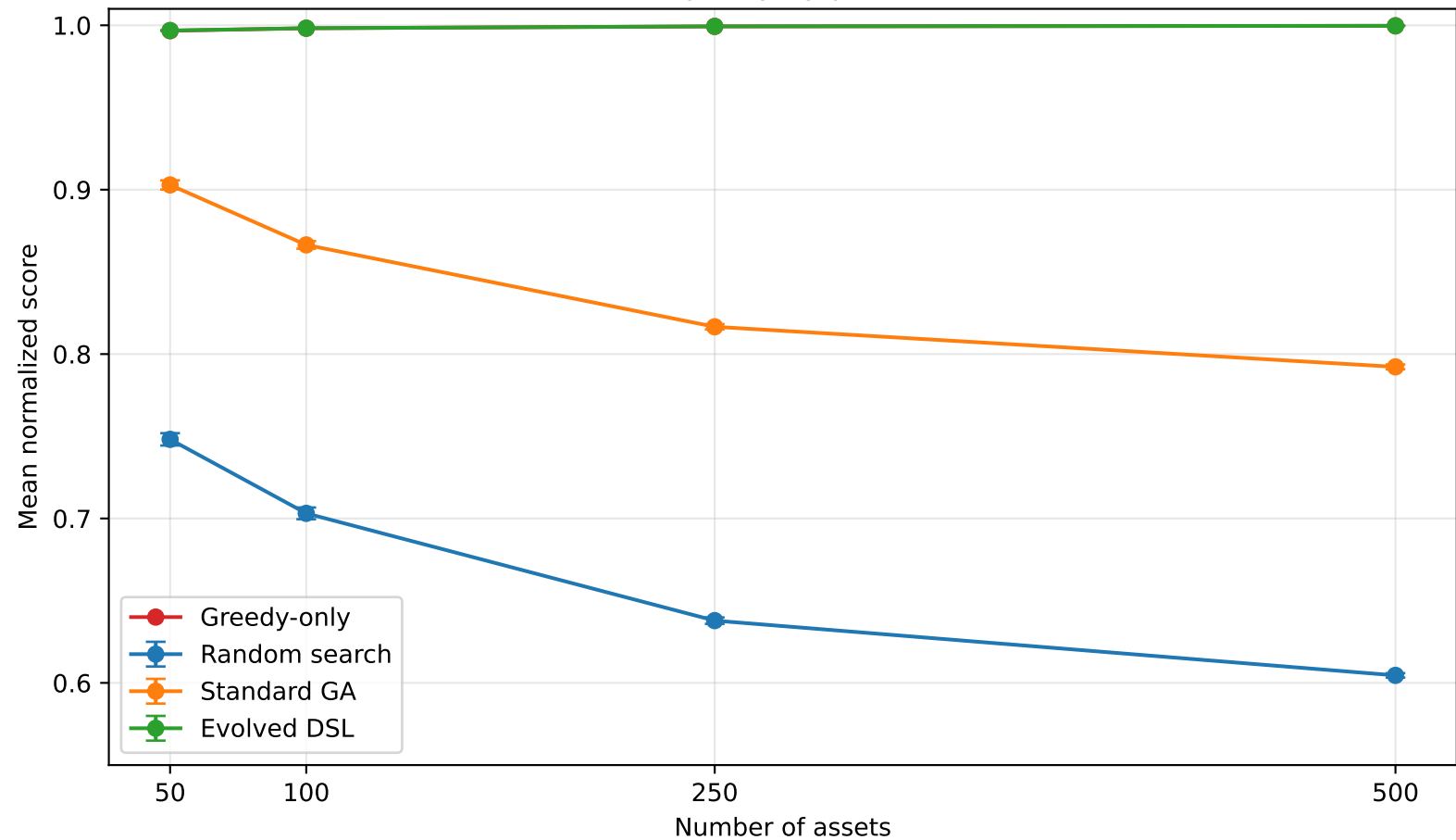
Solution quality by problem size
