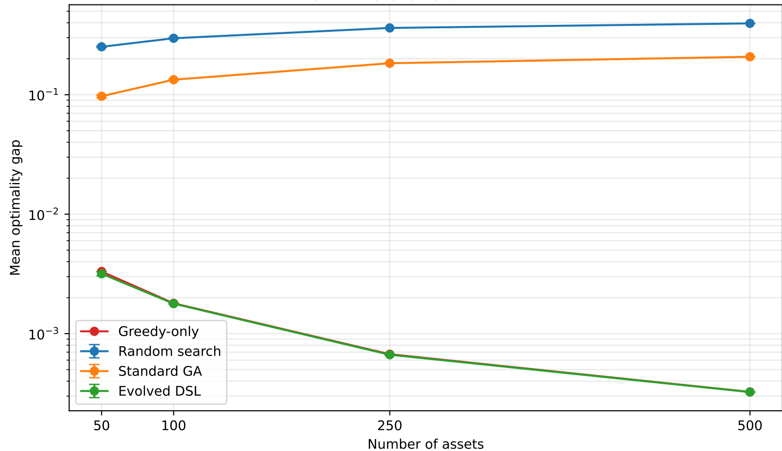
Optimality gap by problem size
