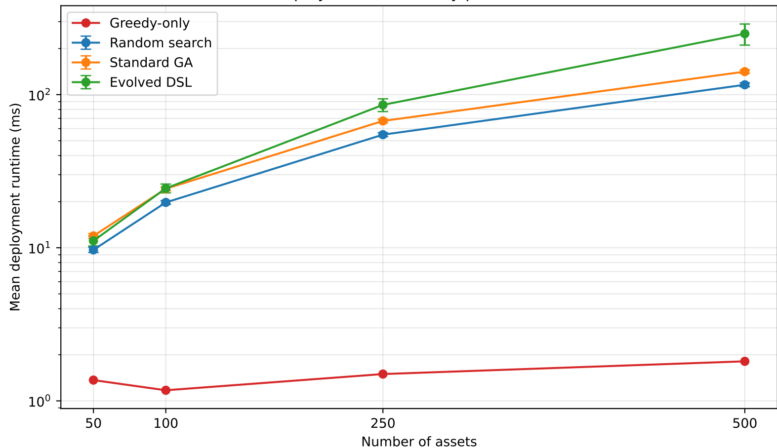
Deployment runtime by problem size
