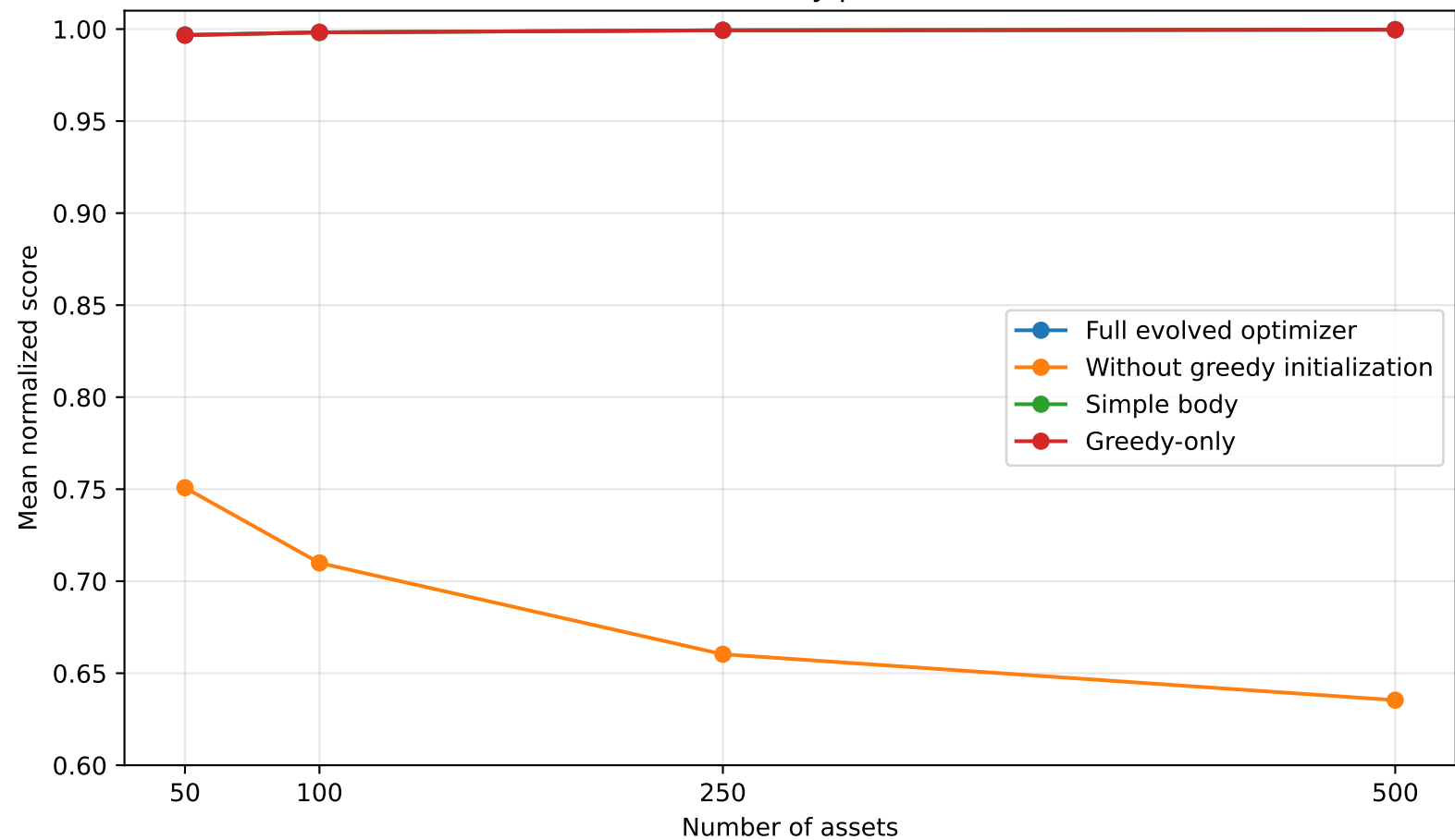
Ablation results by problem size
