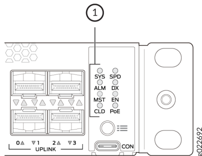
Figure 28: Chassis Status LEDs in EX4100-F Switches
