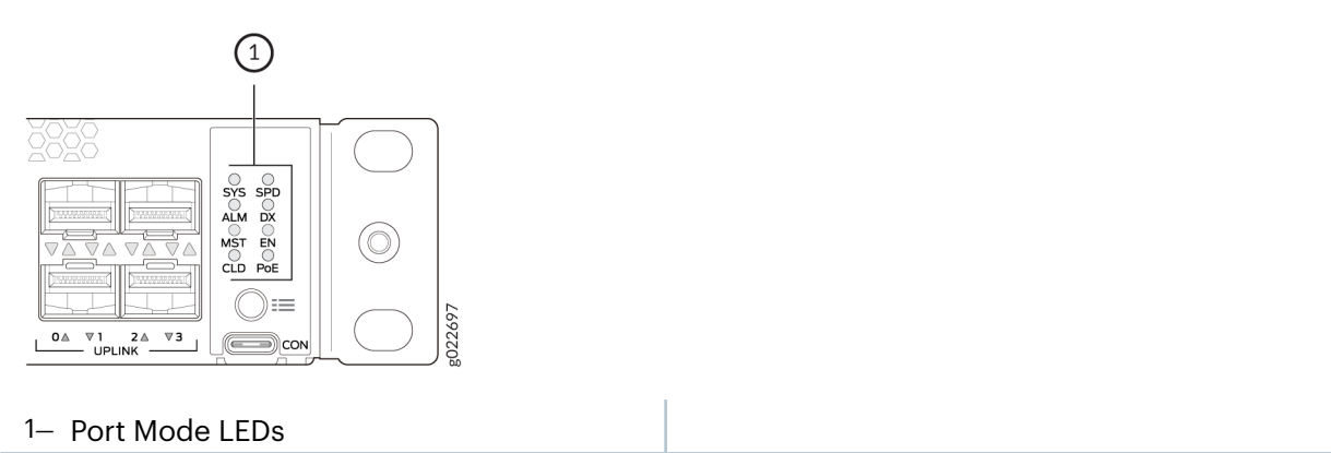
Figure 33: Port Mode LEDs on EX4100-F Switches
