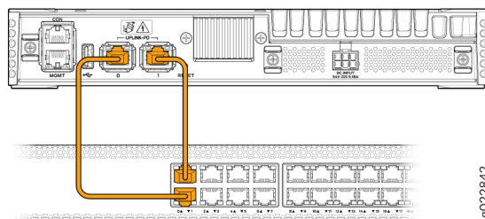
Figure 3: EX4100-F-12P switch connected as a powered device
