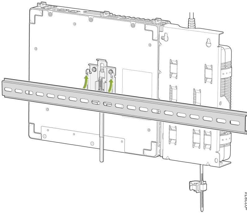
Figure 80: Clipping the DIN Mounting Bracket onto the DIN Rail
