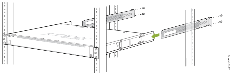
Figure 51: Sliding the Rear-Mounting Blades into the Side Mounting Rails
