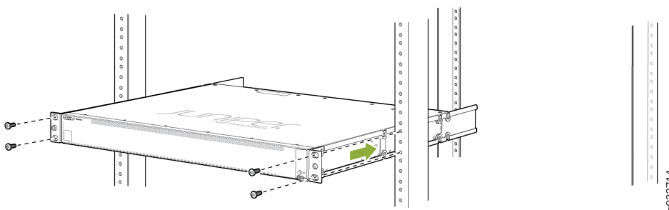
Figure 50: Mounting the Switch to the Front Posts in a Rack
