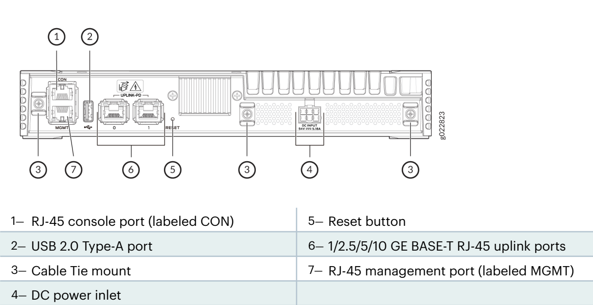
Figure 7: Components on the Rear Panel of the EX4100-F-12P Switch
