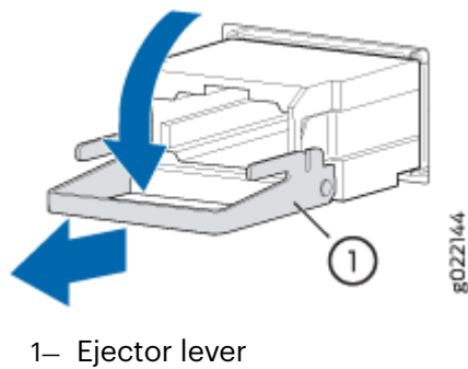
Figure 109: Remove a QSFP+ Transceiver
