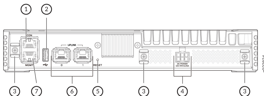
Figure 11: Components on the Rear Panel of the EX4100-F-12T Switch
