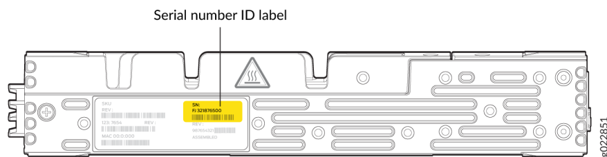
Figure 114: Location of the Serial Number ID Label on the EX4100-F-12P and EX4100-F-12T Switches
