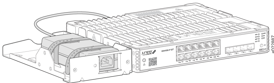
Figure 89: Locking the Power Adaptor Using the Cable Belt - EX4100-F-12T
