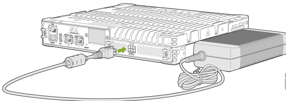
Figure 1: Connect Power Supply Adaptor to DC Inlet of the EX4100-F-12P Switch
