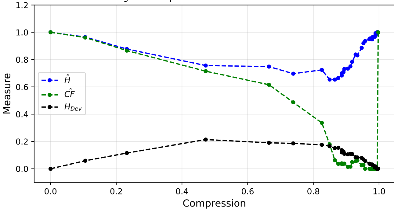
Figure 12: Laplacian RG on NetSci Collaboration
