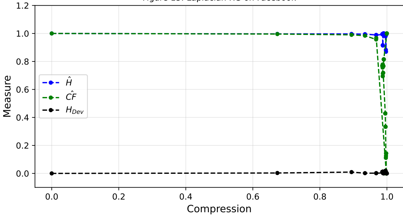
Figure 13: Laplacian RG on Facebook
