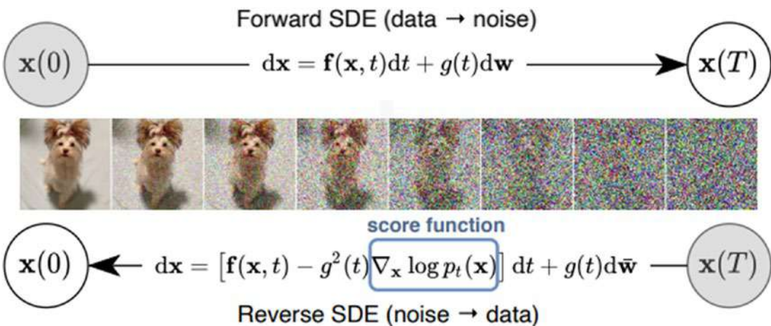
Figure 8-3. Stochastic differential equation (SDE)-based diffusion models
