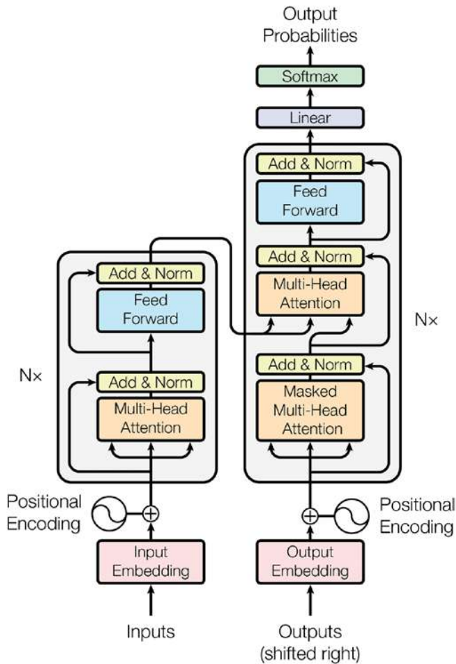
Figure 4-1. The encoder-decoder structure of the Transformer architecture Taken from “ Attention Is All You Need ”
