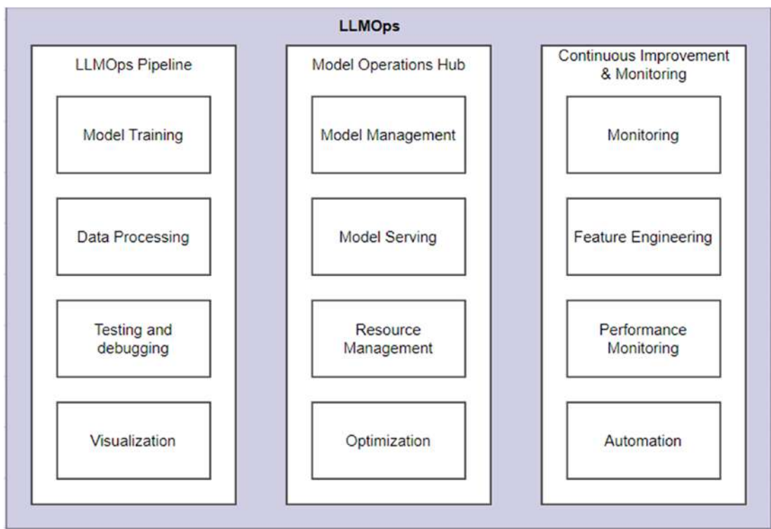
Figure 7-7. LLMOps
