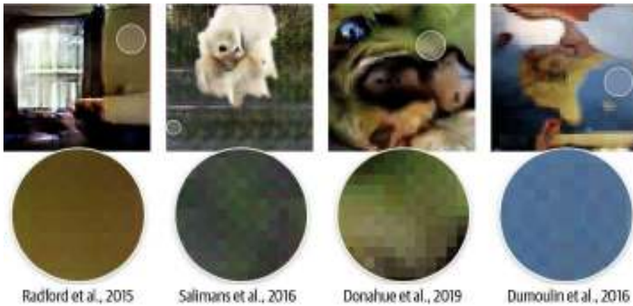
Figure 4-4. Artifacts when using convolutional transpose layers (source: Odena et al., 2016 ) 3
