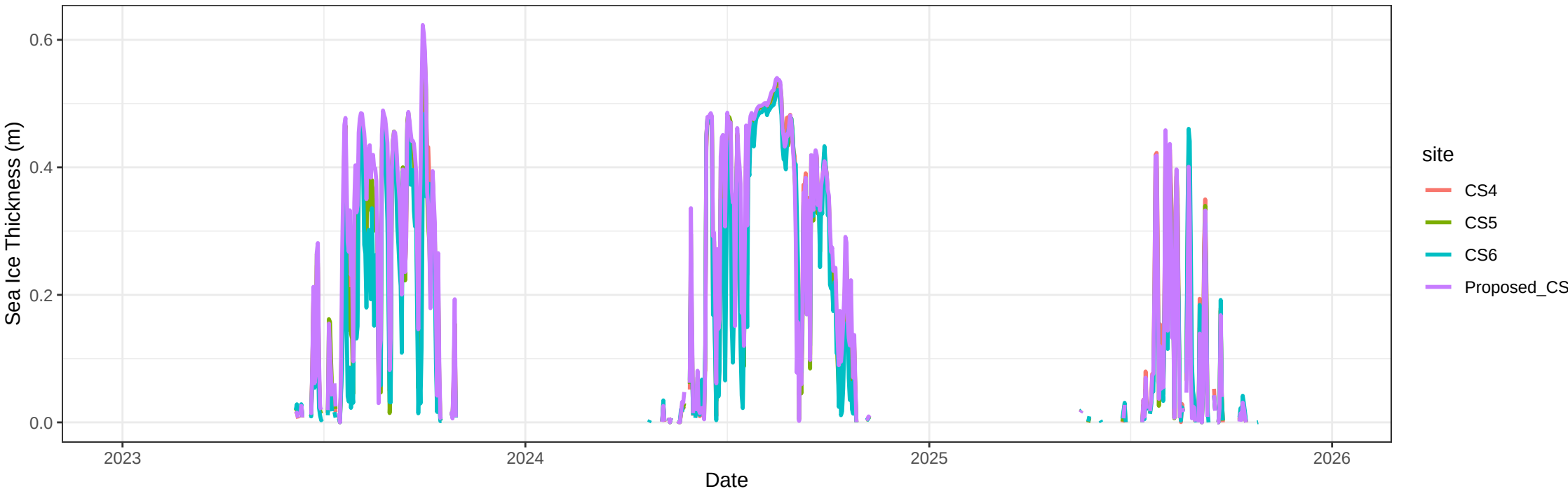
CapeShirreff – Sea Ice Thickness
