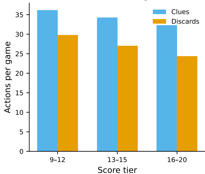
Where turns go
