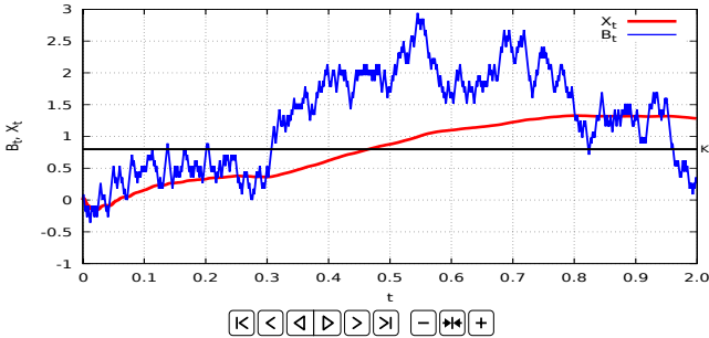
Fig. 13.1: Brownian motion B_t and its moving average X_t .*
