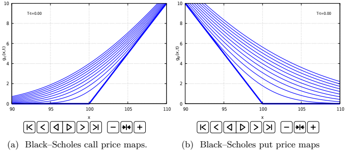
Fig. 6.18: Time-dependent solutions of the Black-Scholes PDE with r = 0 . †
