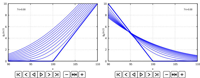
(a) Black–Scholes call price maps.
