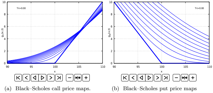
Fig. 6.17: Time-dependent solutions of the Black-Scholes PDE with r = -3\% < 0 . *
