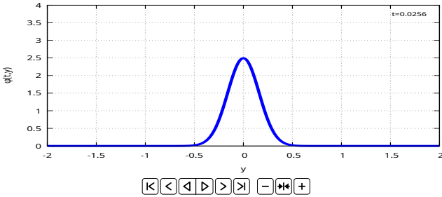
Fig. 6.20: Time-dependent solution of the heat equation.*
