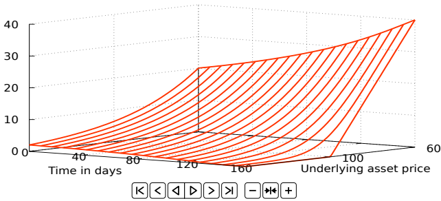
Fig. 6.12: Time-dependent solution of the Black-Scholes PDE (put option).*
