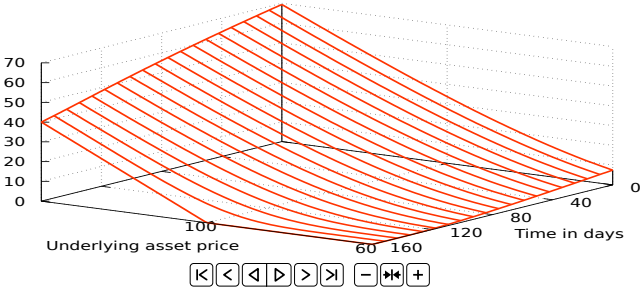
Fig. 6.5: Time-dependent solution of the Black–Scholes PDE (call option).*
