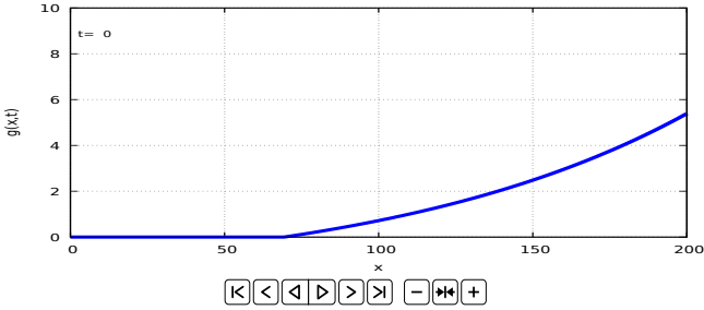
Fig. 6.21: Time-dependent solution of the heat equation.*
