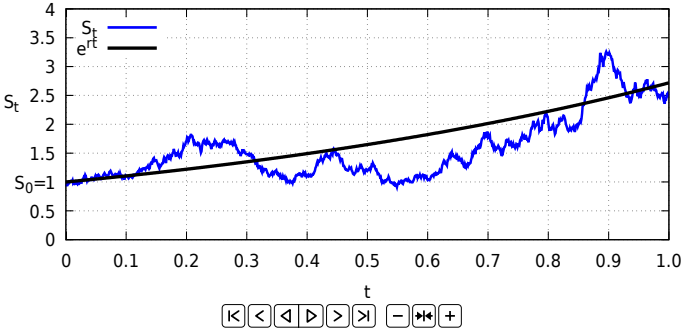
Fig. 5.5: Geometric Brownian motion started at S_0 = 1 , with \mu = r = 1 and \sigma^2 = 0.5 .*
