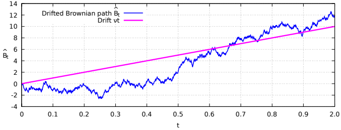
Fig. 7.1: Discretized drifted Brownian path (\hat{B}_t)_{t \geq 0} with \nu > 0 .
