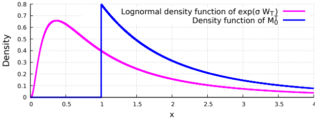
Fig. 10.10: Density of the maximum M_0^T = \text{Max}_{t \in [0, T]} S_t of geometric Brownian motion with S_0 = 1 .
