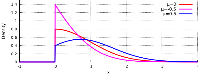
Fig. 10.15: Probability density of the maximum \widehat{X}_0^T of drifted Brownian motion.
