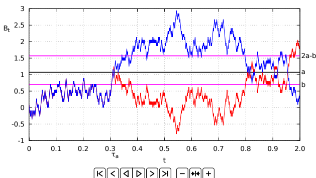
Fig. 10.12: Reflected Brownian motion with a = 1.07 .*
