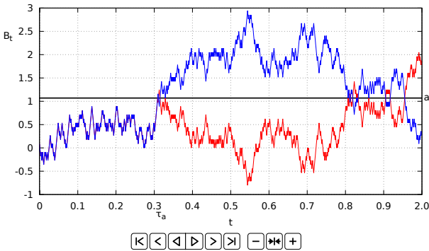
Fig. 10.8: Reflected Brownian motion with a = 1.07 .*
