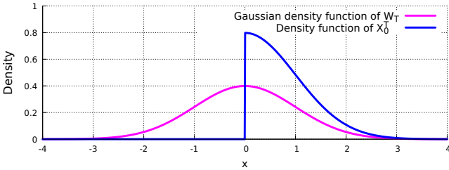
Fig. 10.9: Probability density of the maximum X_0^1 of Brownian motion over [0,1] .
