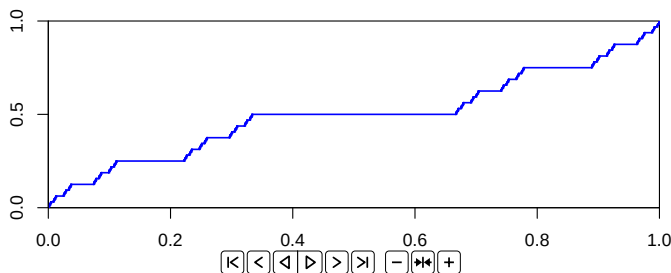
Fig. 10.6: Graph of the Cantor function. †
