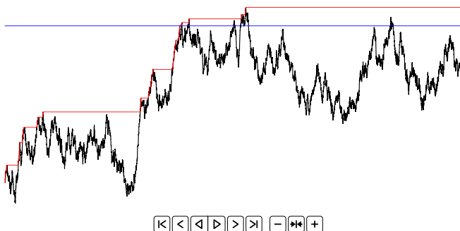
Fig. 10.2: Running maximum of Brownian motion.*
