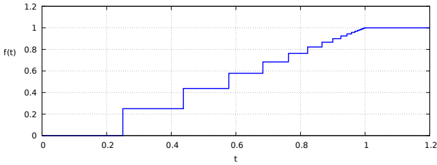
Fig. 10.7: A function with no last point of increase before t = 1 .
