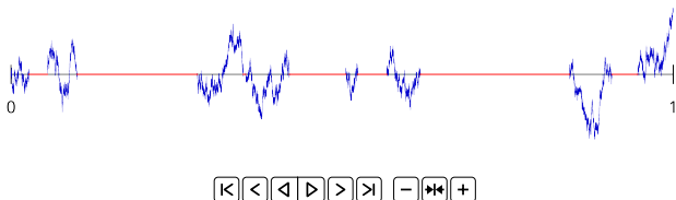
Fig. 10.5: Zeroes of Brownian motion
