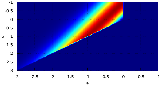
Fig. 10.14: Heat map of the joint density of W_1 and its maximum \hat{X}_0^1 over [0,1] .
