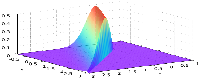
Fig. 10.13: Joint probability density of W_1 and the maximum X_0^1 over [0, 1] .
