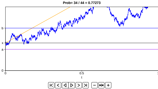
Fig. 14.8: Hitting probabilities of drifted Brownian motion.*
