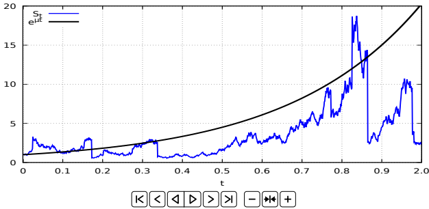
Fig. 20.17: Geometric Brownian motion with compound Poisson jumps.*
