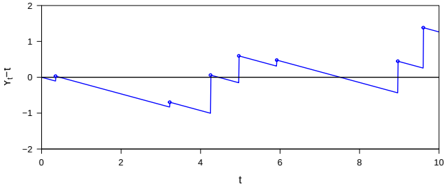
Fig. 20.7: Sample path of a compensated compound Poisson process (Y_t - \lambda t \mathbb{E}[Z])_{t \geq 0} .
