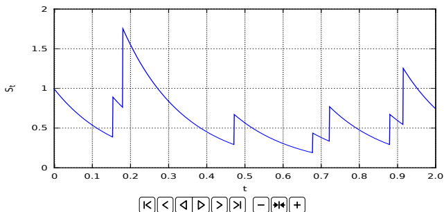
Fig. 20.14: Geometric Poisson process.*
