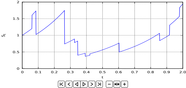
Fig. 20.16: Geometric compound Poisson process.*
