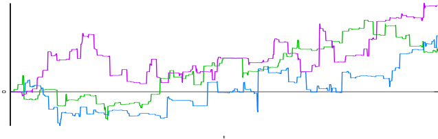
Fig. 20.9: Sample trajectories of a variance gamma process.
