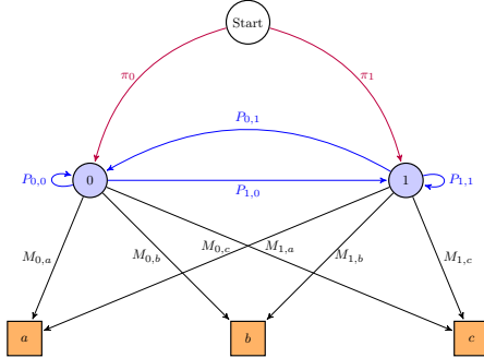
Fig. 9.3: Hidden Markov graph.
