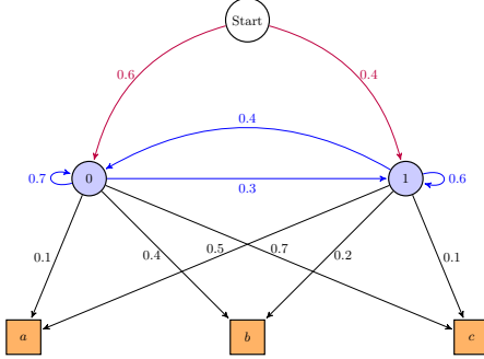
Fig. 9.4: Hidden Markov graph.
