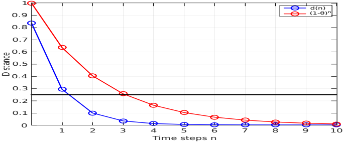
Fig. 6.6: Graphs of distance to stationarity d(n) and upper bound (1 - \theta)^n with \alpha = 1/4 .
