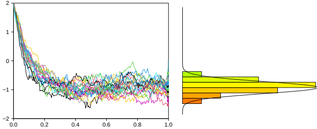
Fig. 6.1: Convergence in distribution.
