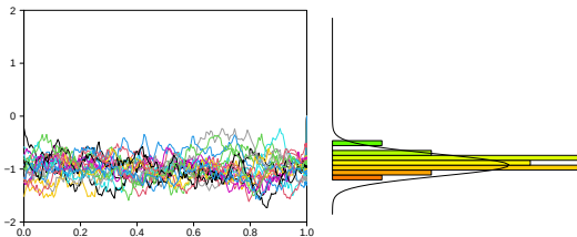
Fig. 6.2: Stationarity in distribution.
