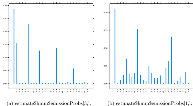
Fig. 9.8: Plots of emission probabilities.
