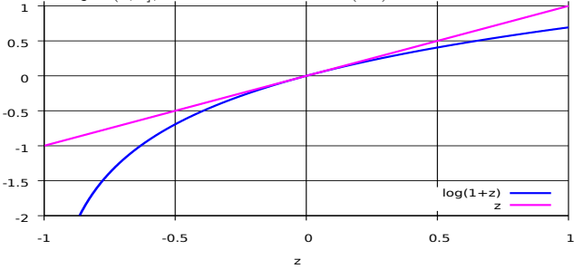
Fig. 5.2: Log function.
