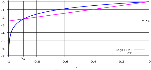
Fig. 5.3: log function.
