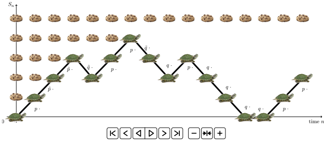
Fig. 5.1: Random walk with cookies.*
