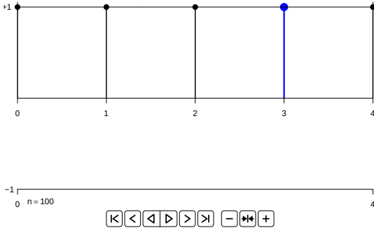
Fig. 7.3: Simulation with N = 3 , p = \sqrt{0.75} \approx 0.87 , \beta = -0.47 , and z_0 = z_4 = +1 .*
