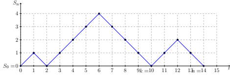
Fig. 4.7: Last return to state 0 at time k = 10 .
