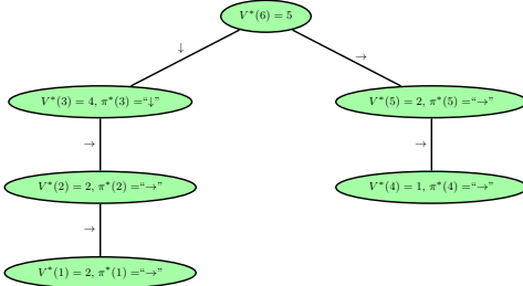
Fig. 10.3: Optimal policies.
