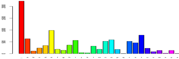
Fig. 9.7: Frequency analysis of alphabet letters.
