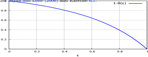
Fig. 8.2: Graph of 1 - \theta(\varepsilon) as a function of \varepsilon \in [0, 1] .
