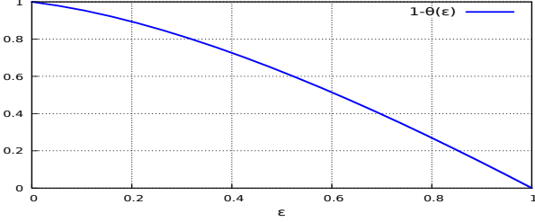
Fig. 8.6: Graph of 1 - \theta(\varepsilon) as a function of \varepsilon \in [0, 1] .
