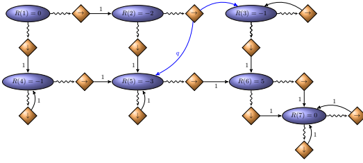
Fig. 10.4: Stochastic MDP.
