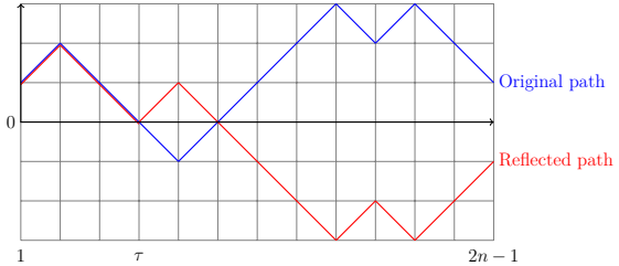
Fig. 4.5: Random walk and reflected path.
