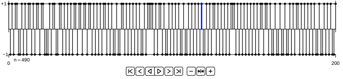
Fig. 7.2: Simulation of the Ising model with N = 199 , p = 0.02 , and z_0 = z_{N+1} = +1 .*
