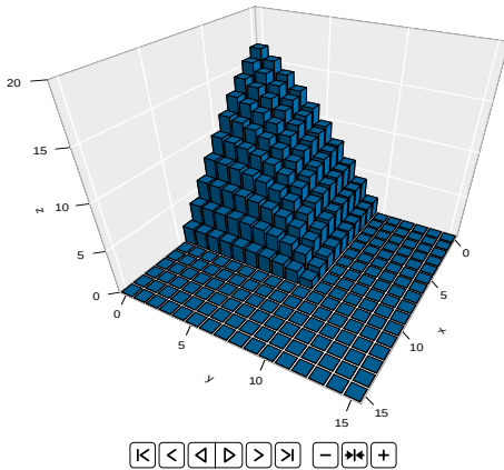
Fig. S.1: Backward solution of Equation (S.24) for \mu_A(x, y) with N = 10 .*
