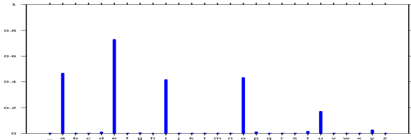
Fig. 9.6: Enhanced classification.
