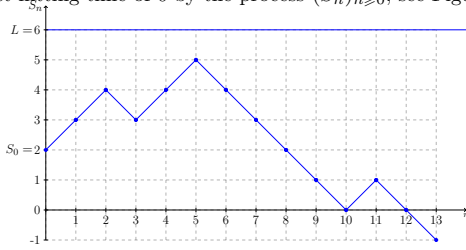
Fig. 1.2: Sample path of the random walk (S_n)_{n \geqslant 0} .
