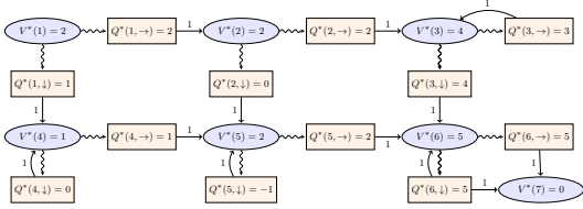
Fig. 10.1: Action-value functional.
