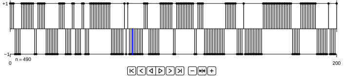
Fig. 7.1: Simulation of the Ising model with N = 199 , p = 0.98 , and z_0 = z_{N+1} = +1 . †
