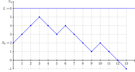
Fig. 4.8: Sample path of the random walk (S_n)_{n \geq 0} .
