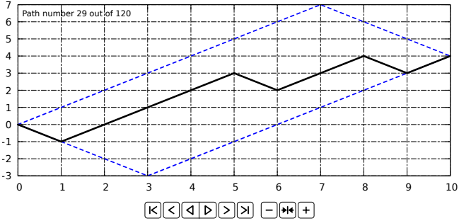
Fig. 4.1: Graph of 120 = \binom{10}{7} = \binom{10}{3} paths linking (0,0) to (10,4) .*
