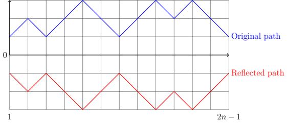
Fig. 4.4: Random walk and reflected path.
