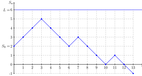
Fig. 4.6: Sample path of the random walk (S_n)_{n \geq 0} .
