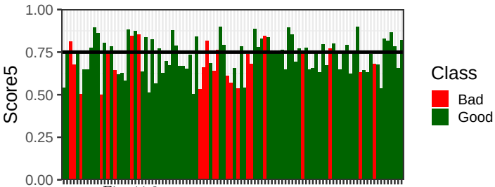
Fig. 11.8: Logistic regression output on 5 criteria.
