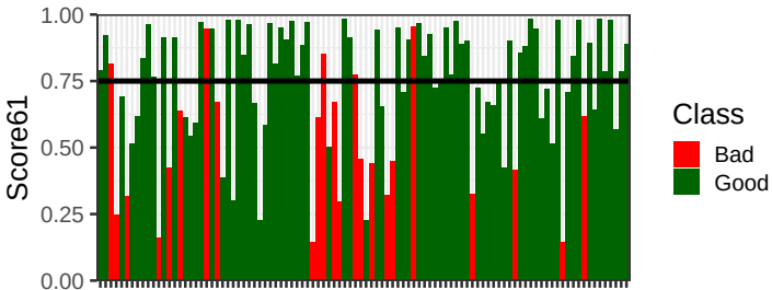
Fig. 11.9: Logistic regression output on 61 criteria.
