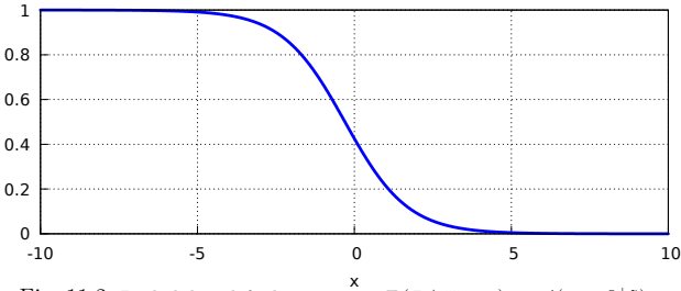
Fig. 11.2: Probability default curve z \mapsto \mathbb{P}(B \mid X = z) = 1/(1 + e^{a+z}) .
