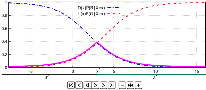
Fig. 11.4: Animated graph of optimal decision rule.*
