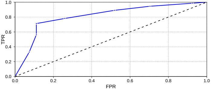
Fig. 11.10: ROC curve.
