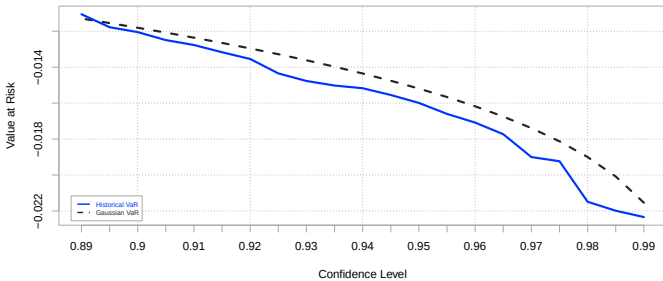
Fig. 7.5: Historical vs. Gaussian estimates of Value at Risk.
