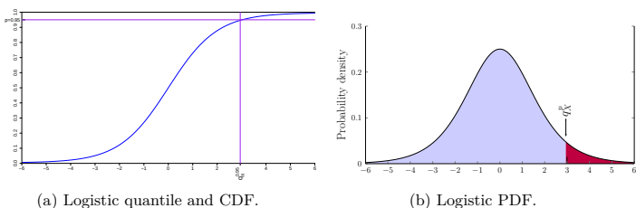
Fig. 7.12: Logistic CDF and PDF.
