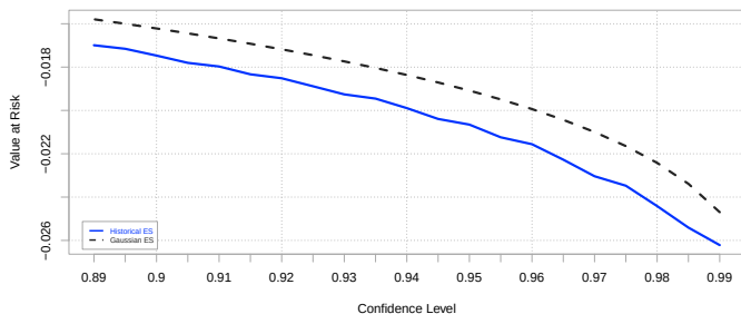
Fig. 7.6: Historical vs. Gaussian estimates of Expected Shortfall.
