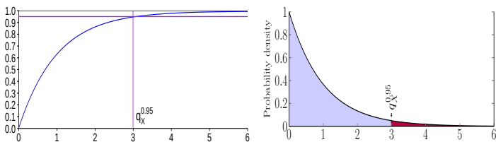
(a) Exponential quantile and CDF.
