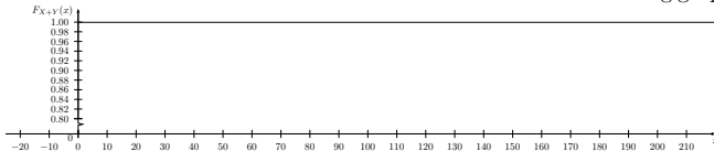
Fig. 7.11: Cumulative distribution function of X + Y .
