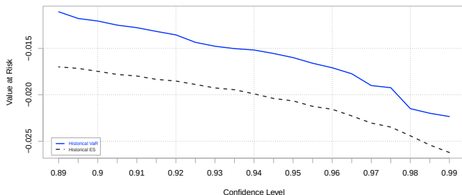
Fig. 7.4: Value at Risk vs. Expected Shortfall.
