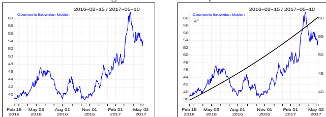
Fig. 1.15: Graph of simulated geometric Brownian motion.
