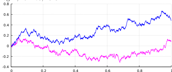
Fig. 1.3: Two sample paths of one-dimensional Brownian motion.
