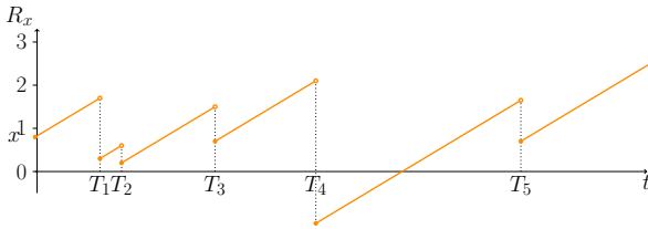
Fig. 3.9: Sample path (with ruin) of a reserve process (R_x(t))_{t \in \mathbb{R}_+} .
