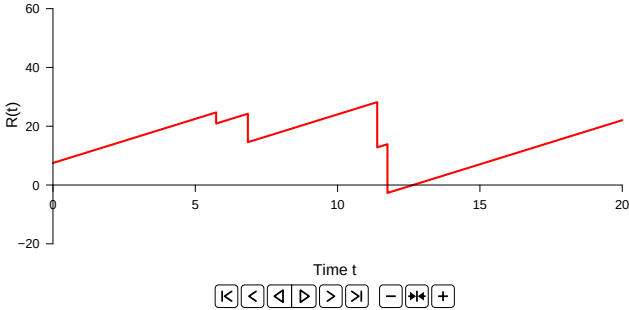
Fig. 3.10: Sample paths of a reserve process (R_x(t))_{t \in \mathbb{R}_+} .*
