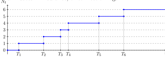
Fig. 3.1: Sample path of a counting process (N_t)_{t \in \mathbb{R}_+} .
