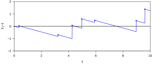
Fig. 3.7: Sample path of a compensated compound Poisson process (Y_t - \lambda t \mathbb{E}[Z])_{t \geq 0} .
