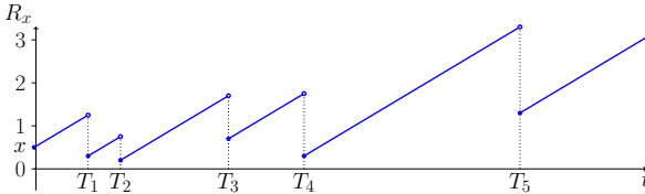
Fig. 3.8: Sample path (without ruin) of a reserve process (R_x(t))_{t \in \mathbb{R}_+} .
