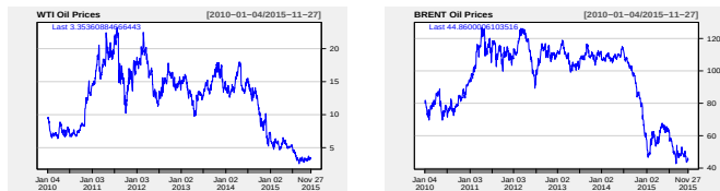
(a) WTI price graph.
