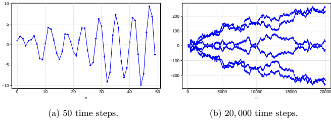
Fig. 2.9: Nonstationarity of an AR(2) time series with \alpha_1 = 1 and \alpha_2 = -1 .
