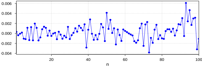
Fig. 2.5: ARCH(2) Samples.
