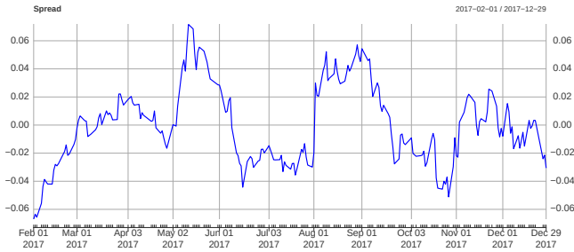
Fig. 2.20: Spread graph.
