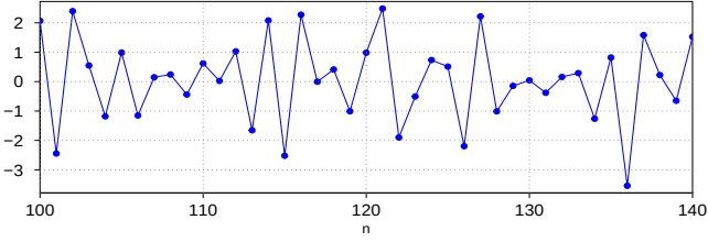
Fig. 2.1: MA(2) Samples.
