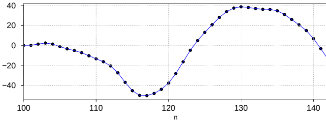
Fig. 2.4: ARIMA(1, 2, 3) Samples.
